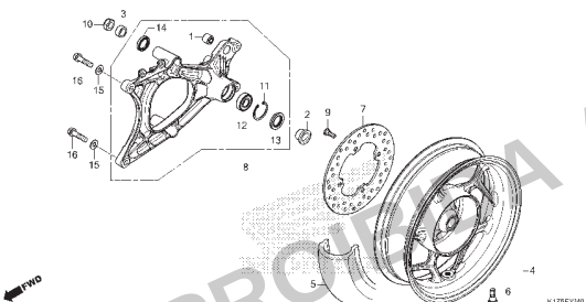
C-22.40 Roda Traseira • Garfo Traseiro (PCX160A)
